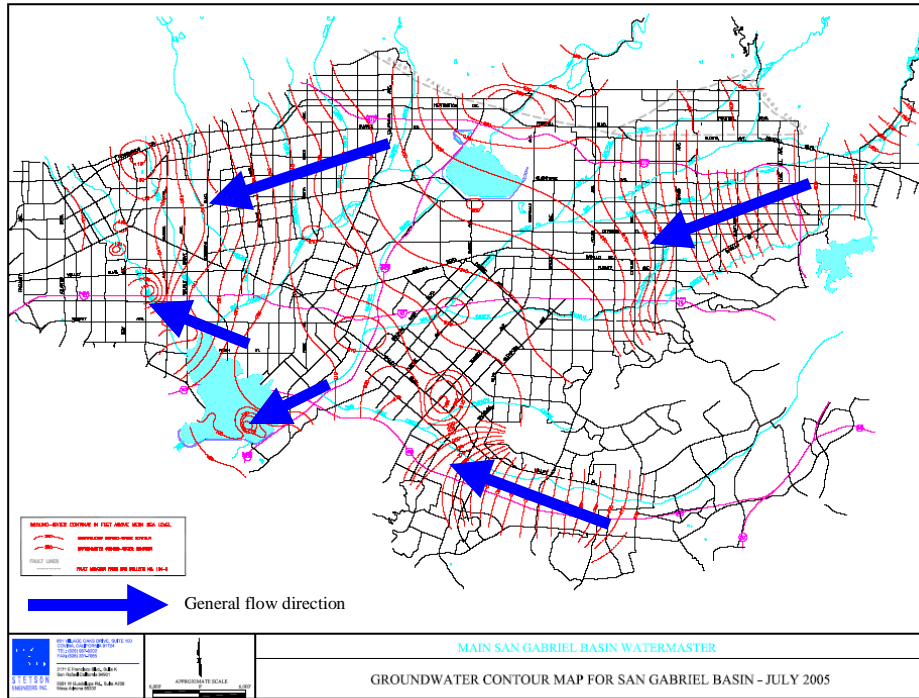
Figure 7-7 Groundwater Contour Map of the Main San Gabriel and Puente Basins – Summer 2005
